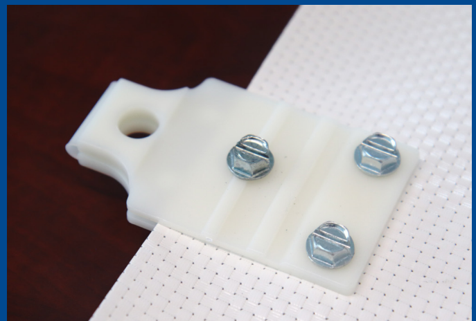
Nylon one-piece clips securely retain fabric with only 3 #14 x 1/2" sheet metal screws
